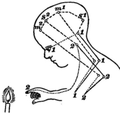
FIG. 4. —The dotted lines stand for affr. ent paths the broken lines for paths between the centres; the entire lines for efferent paths.
