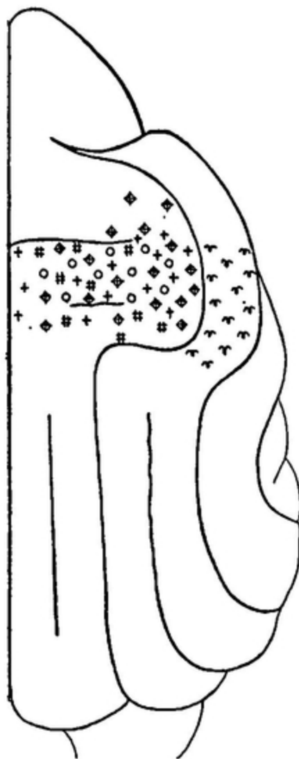
FIG. 21.—Dog's motor centres, right hemisphere, according to Paneth.— The points of the motor region are correlated as follows with muscles: the loops with the orbicularis palpebrarum; the plain crosses with the flexor, the crosses inscribed in circles with the extensor, digitorum communis of the fore-paw; the plain circles with the abductor pollicis longus; the double crosses with the extensor communis of the hind-limb.
