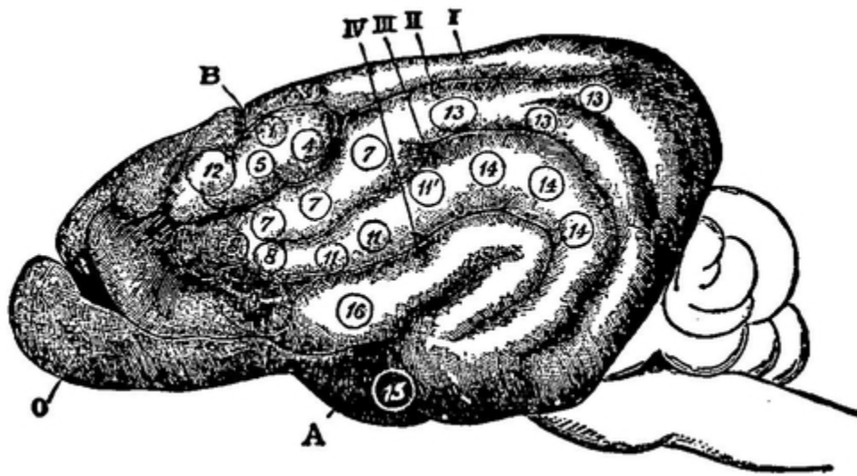
FIG. 5. —Left Hemisphere of Dog's Brain, after Ferrier. A, the fissure of Sylvius. B, the crucial sulcus. O, the olfactory bulb. I, II, III, IV, indicate the first, second, third, and fourth external convolutions respectively. (1), (4), and (5) are on the sigmoid gyrus.
