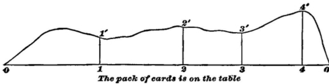
FIG. 29. — The Stream of Consciousness.
