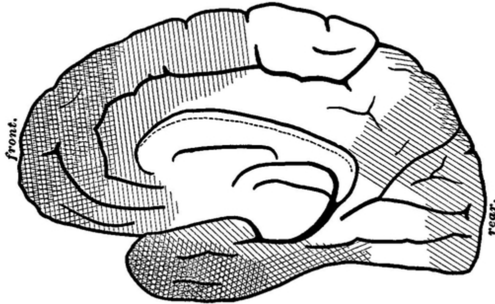
FIG. 9. — Right Hemisphere of Human Brain. Mesial Surface.
