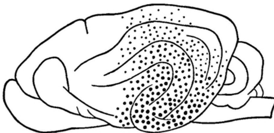
FIG. 16.—Luciani’s Hearing Region.
