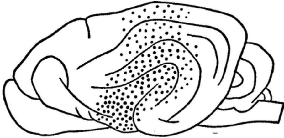
FIG. 19.—Luciani's Olfactory Region in the Dog.
