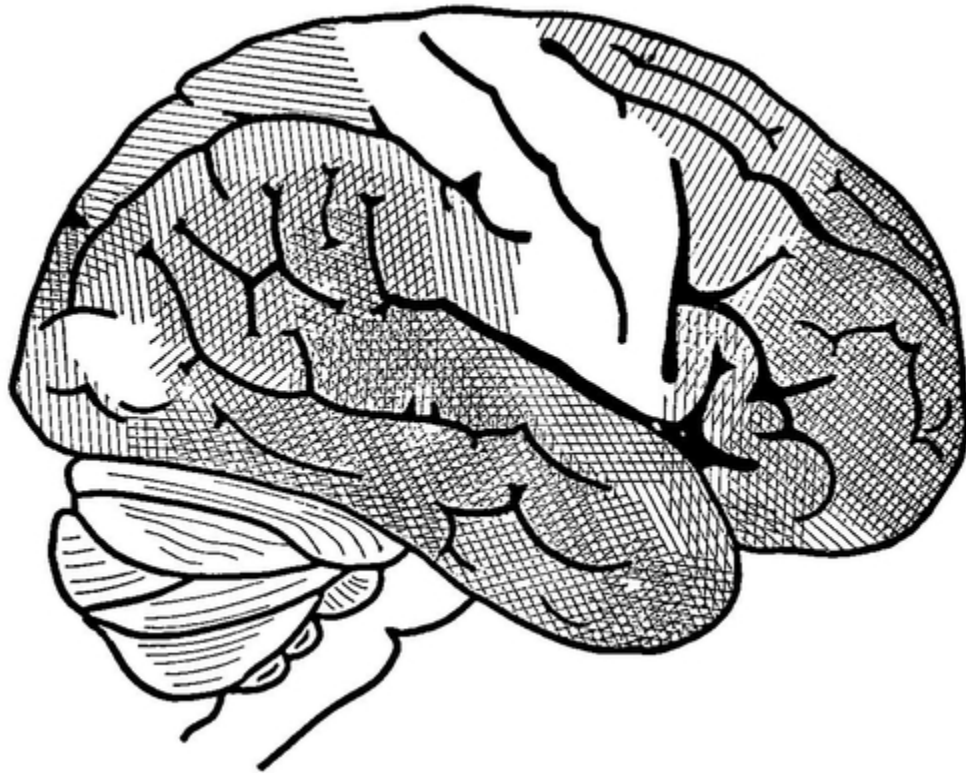
FIG. 8.—Right Hemisphere of Human Brain. Lateral Surface.
