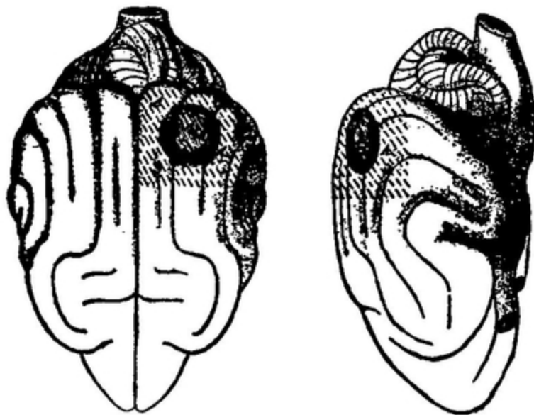
Figs. 12 Figs. 13 The Dog's visual centre according to Munk, the entire striated region, A, A, being the exclusive seat of vision, and the dark central circle, A', being correlated with the retinal centre of the opposite eye.
