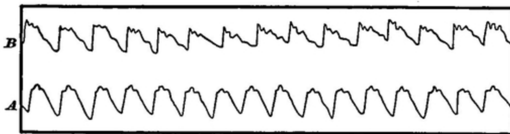
FIG. 23.—Sphygmographic pulse-tracing. A, during intellectual repose ; B, during intellectual activity. (Mosso.)
